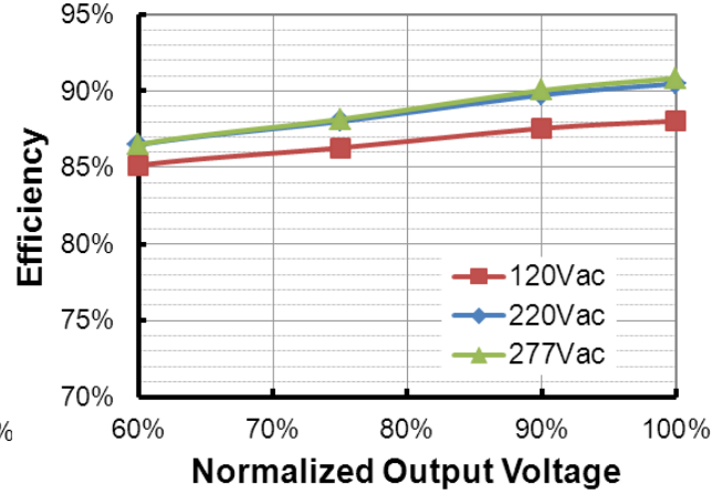
EUD-240S420DVL ( I_o=4200mA ) Efficiency vs. Output Voltage
