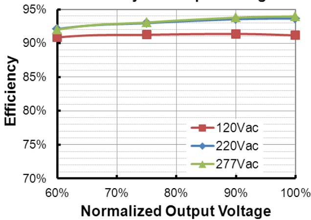
EUD-240S210DVL ( I_o=1400mA ) Efficiency vs. Output Voltage
