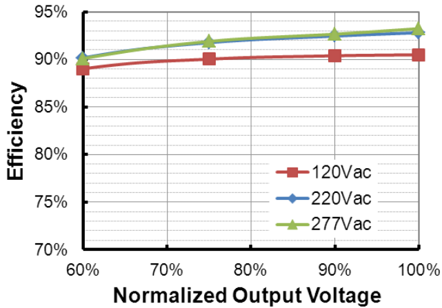
EUD-240S670DVL ( I_o=4450mA ) Efficiency vs. Output Voltage
