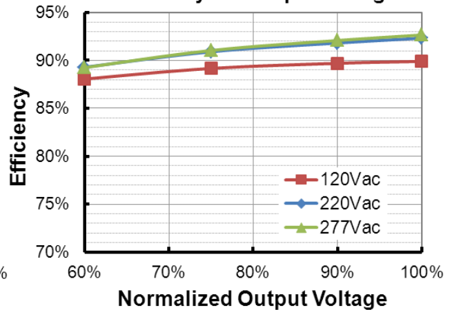
EUD-240S210DVL ( I_o=2100mA ) Efficiency vs. Output Voltage
