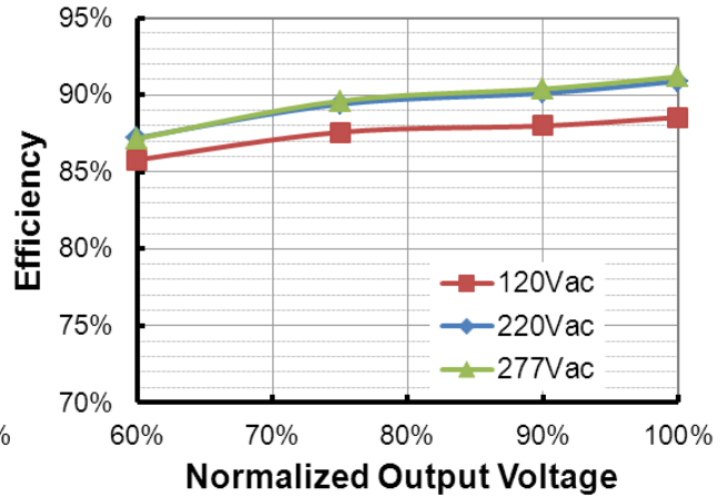
EUD-240S670DVL ( I_o=6700mA ) Efficiency vs. Output Voltage
