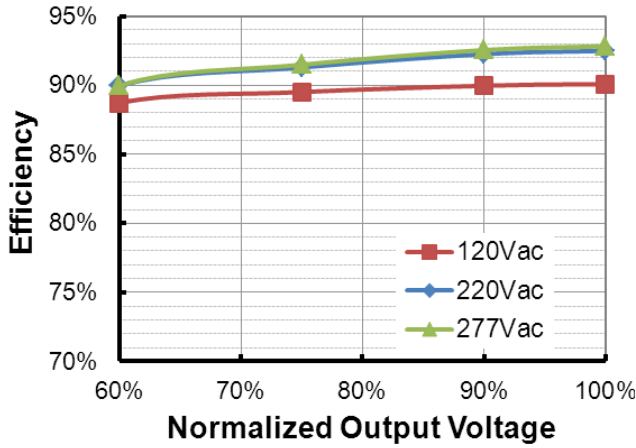
EUD-240S420DVL ( I_o=2800mA ) Efficiency vs. Output Voltage
