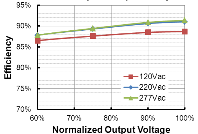
EUD-150S210DVL (I o =2100mA) Efficiency vs. Output Voltage
