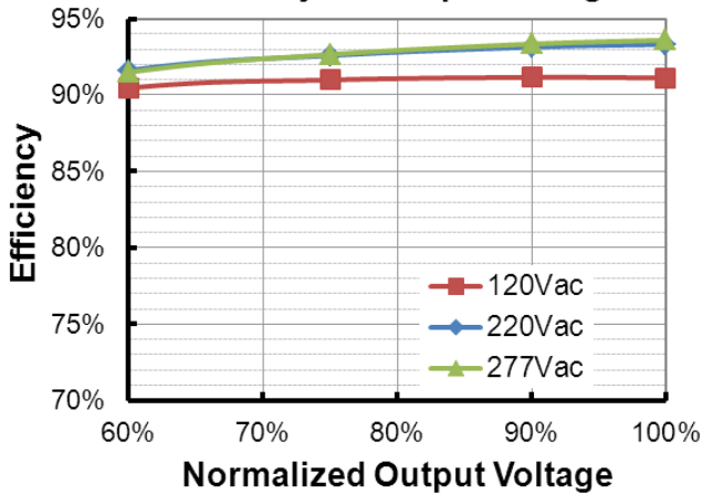
EUD-150S070DVL (I o =450mA) Efficiency vs. Output Voltage
