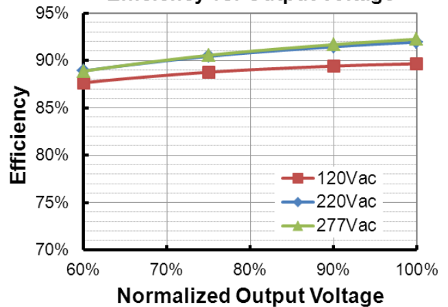
EUD-150S105DVL (I o =1050mA) Efficiency vs. Output Voltage
