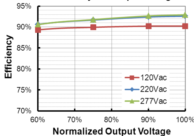
EUD-150S210DVL (I o =1400mA) Efficiency vs. Output Voltage
