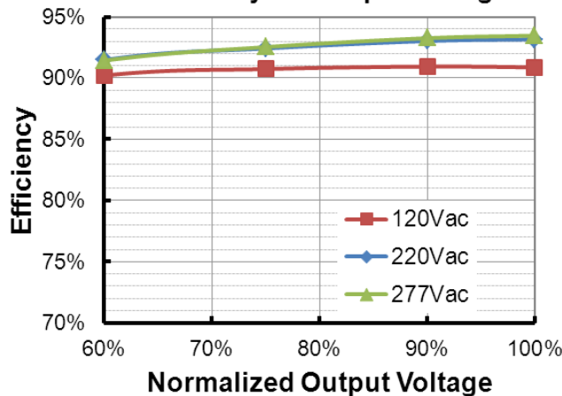
EUD-150S105DVL (I o =700mA) Efficiency vs. Output Voltage
