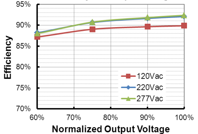
EUD-150S070DVL (I o =700mA) Efficiency vs. Output Voltage
