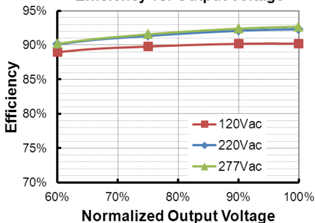
EUD-096S105DVL (I o =700mA) Efficiency vs. Output Voltage
