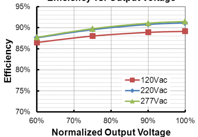
EUD-096S105DVL (I o =1050mA) Efficiency vs. Output Voltage
