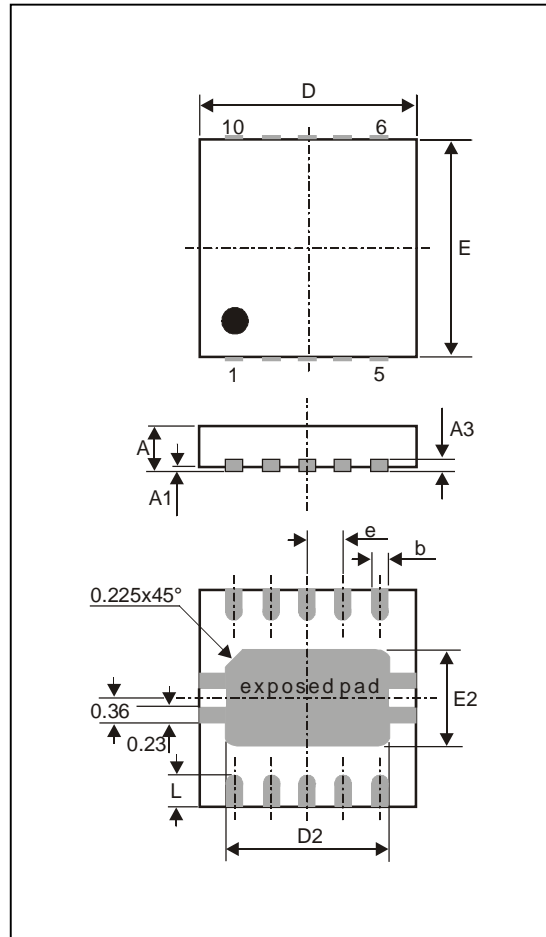
Fig. 19: 10L MLPD 3x3 (Micro Leadframe Package Dual)
